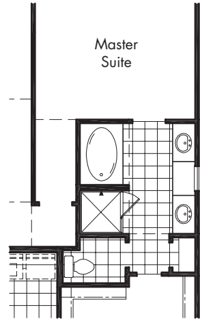
Separate Shower Master Bath Upgrade Option 1300-90
