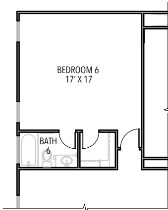
OPTIONAL BEDROOM 6 WITH BATH 6
