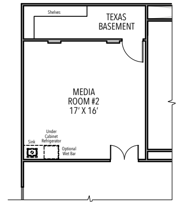
OPTIONAL MEDIA ROOM #2
