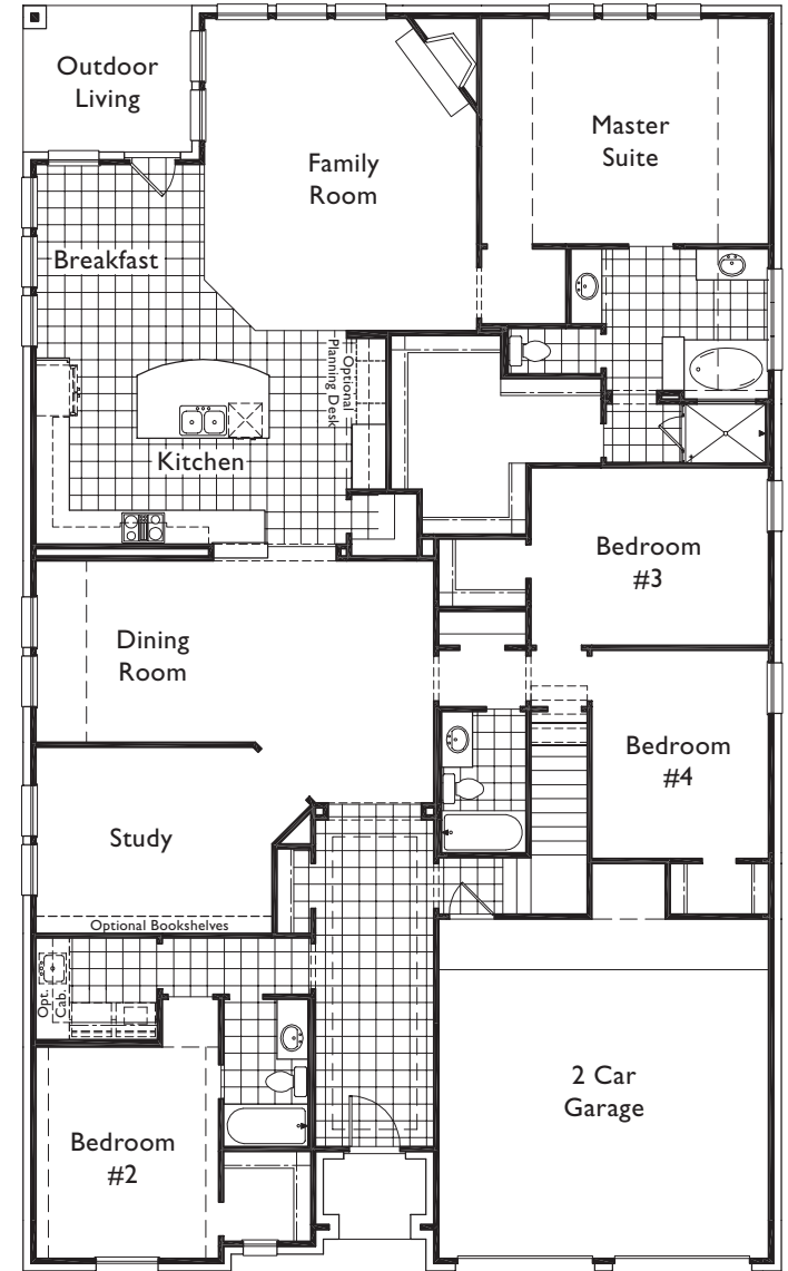
Lower Level with Staircase for Upper Level Options
