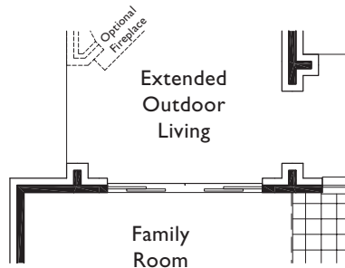
Sliding Doors at Outdoor Living Option 1400-52
