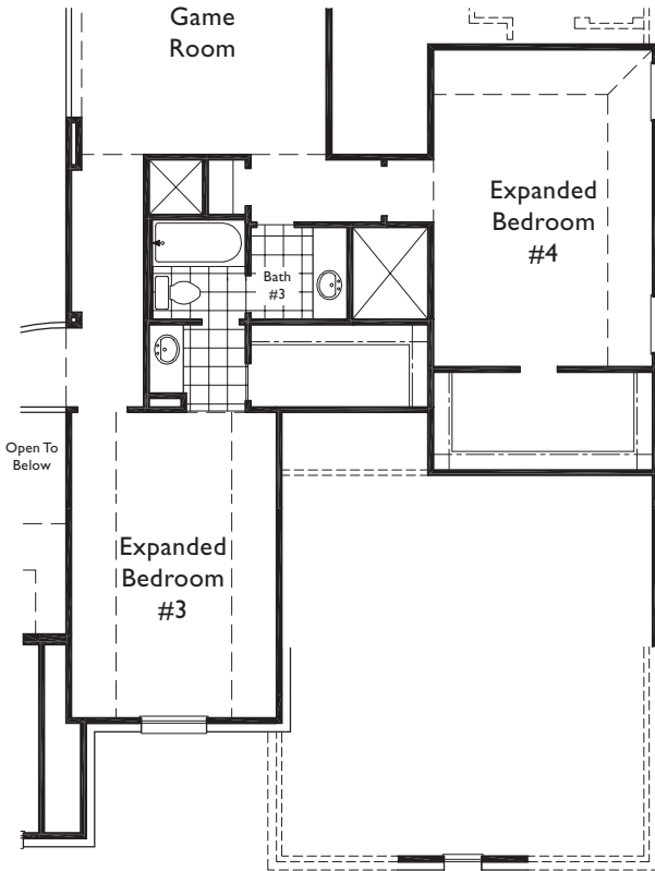
Expanded Bedrooms #3 and #4 Option in lieu of Bedroom #3 ~ Lifestyle Room 2000-75
